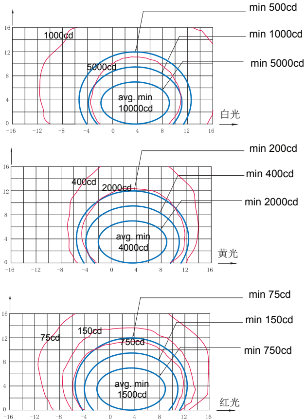
跑道边灯, ICAO 图A2-10
